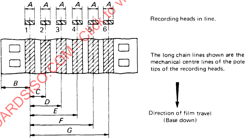
FIGURE — Location and dimensions of the magnetic sound recording head gaps
