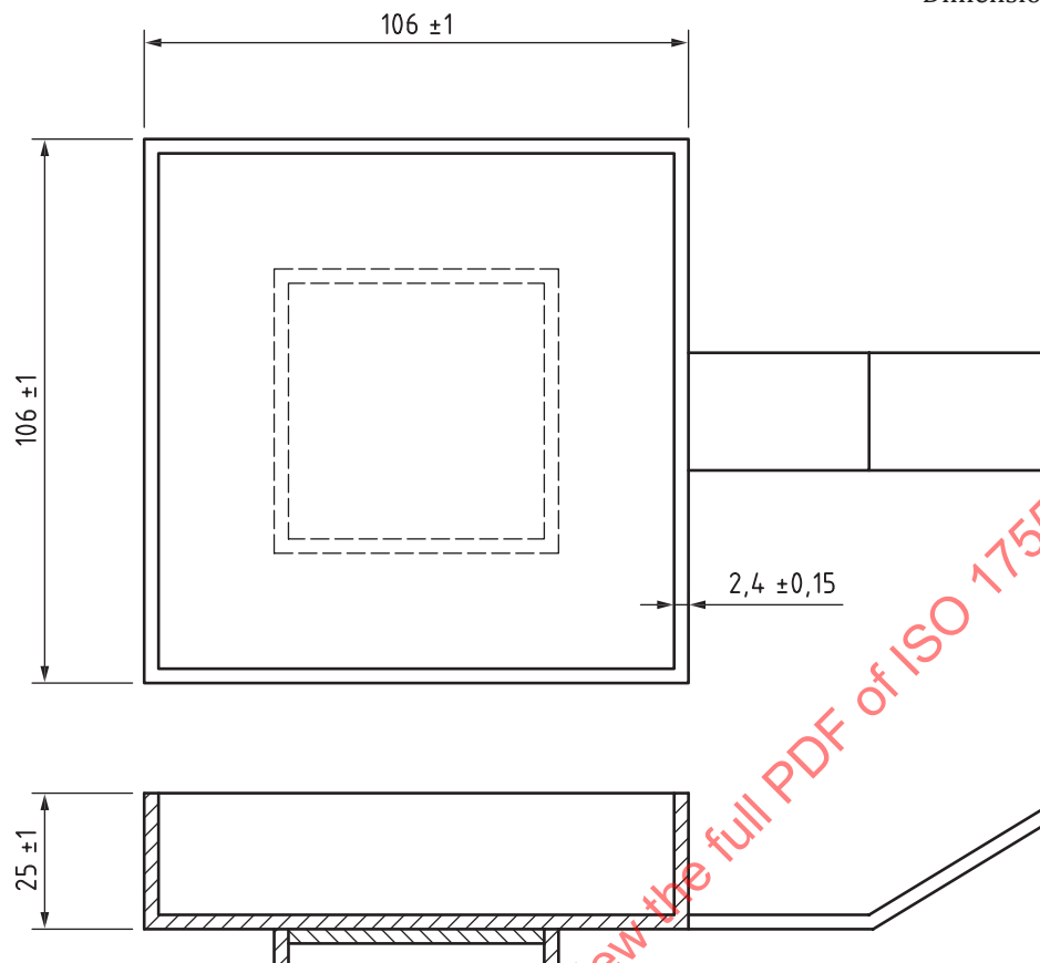
Figure 3 — Specimen holder
