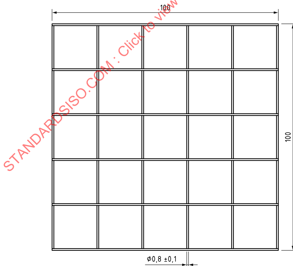
Figure 5 — Fine wire grid made from 0,8 mm wire
