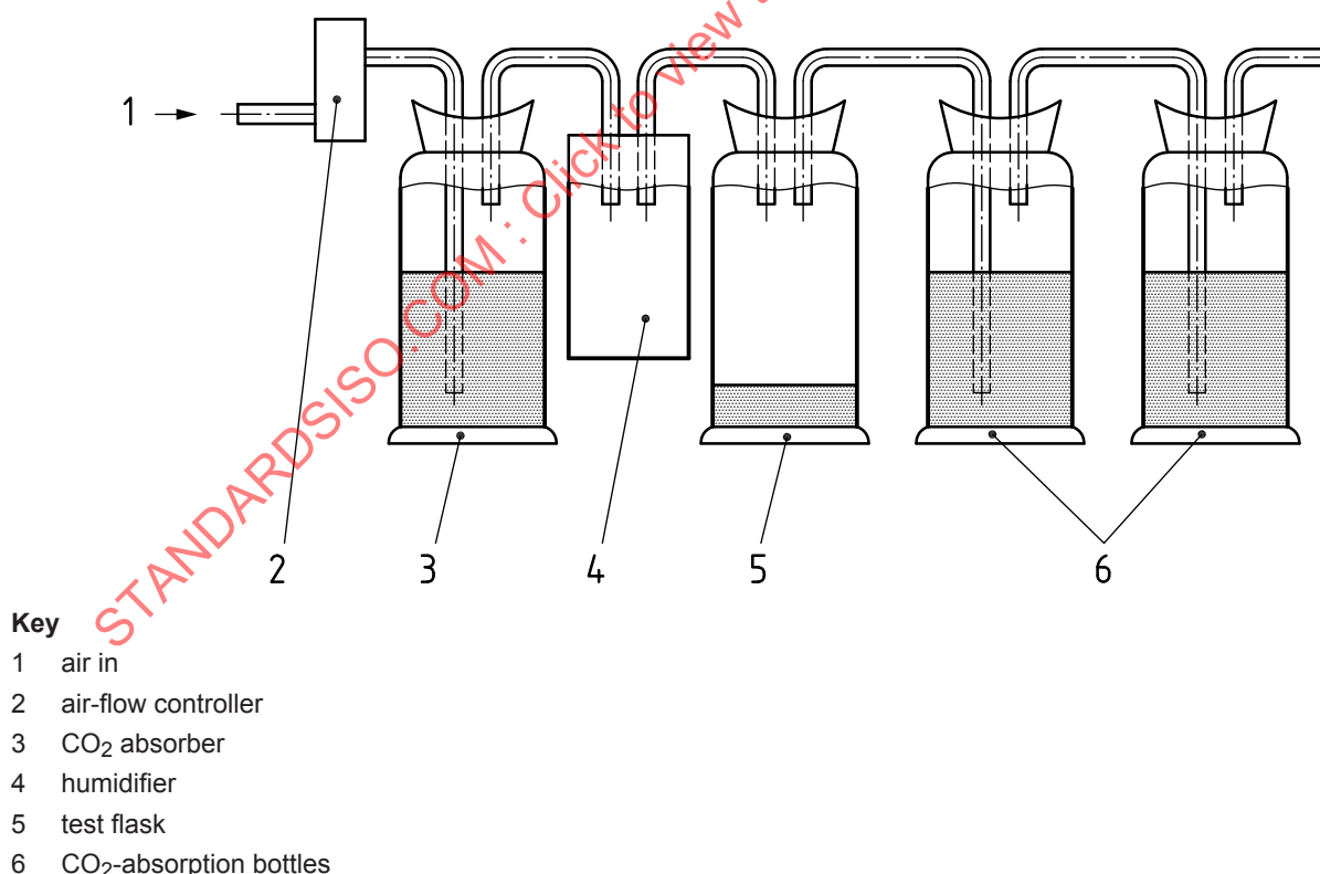
Figure B.1 — Schematic diagram of a system for measuring the amount of carbon dioxide evolved
