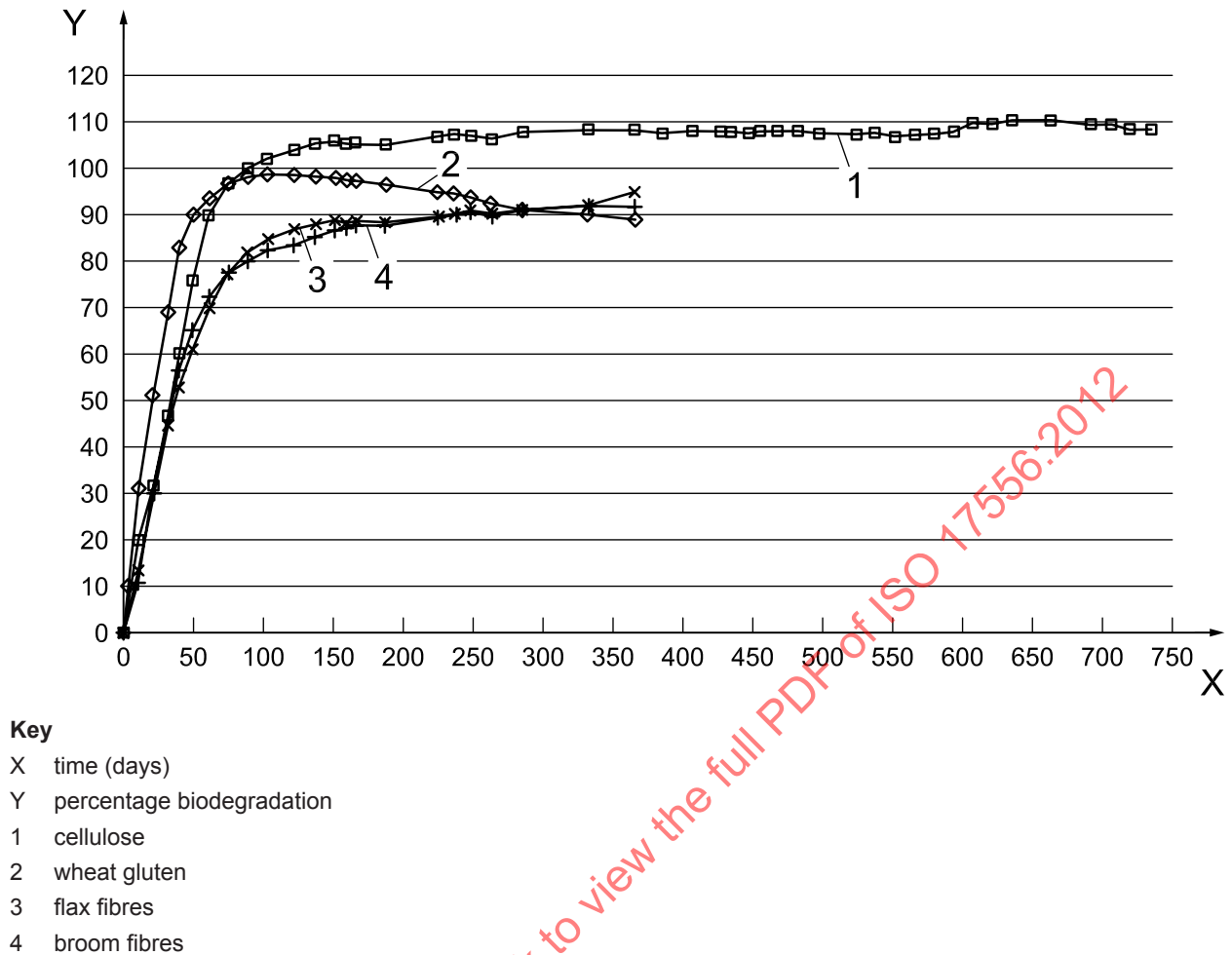
Figure F.1 — Evolution of the biodegradation of cellulose, wheat gluten, flax fibres and broom fibres in soil
