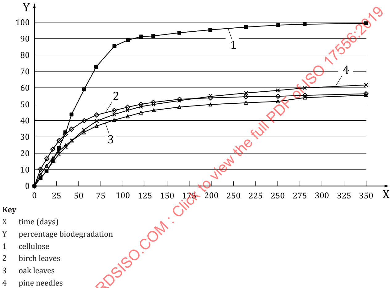
Figure F.2 — Evolution of the biodegradation of cellulose, birch leaves, oak leaves and pine needles in soil
