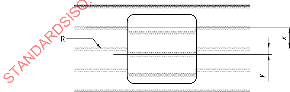
Figure 1 — Schematic drawing of interference fringes at a crater ( n = 0 )
