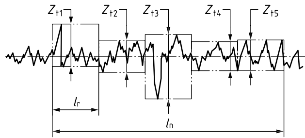
Figure B.3 — Determination of the average surface roughness R_{Z5}
