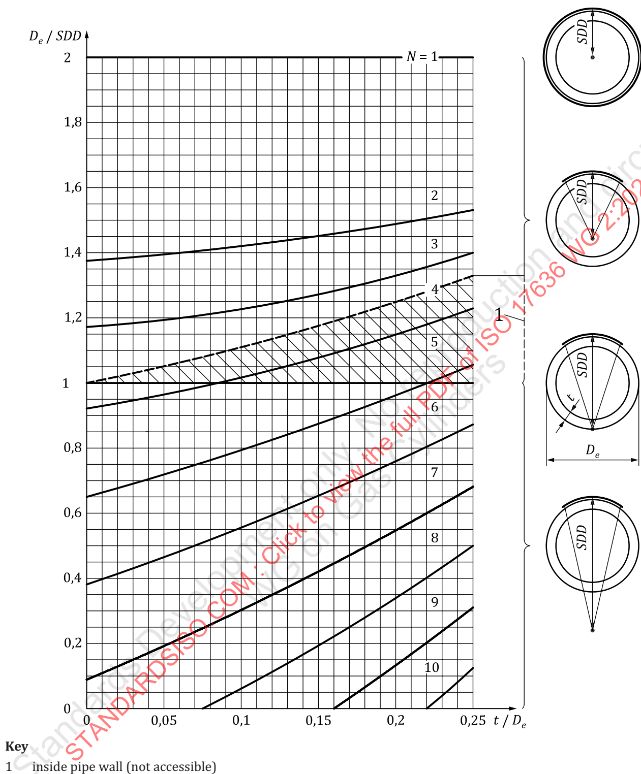
Figure A.2 — Minimum number of exposures, N , for off-centre penetration with source inside and for double-wall penetration considering a maximum permissible increase in penetrated thickness \Delta t/t = 10\% (testing class B) as a function of ratios t/D_e and D_e/SDD , due to inclined penetration in the evaluable areas of sufficient SNR_N
