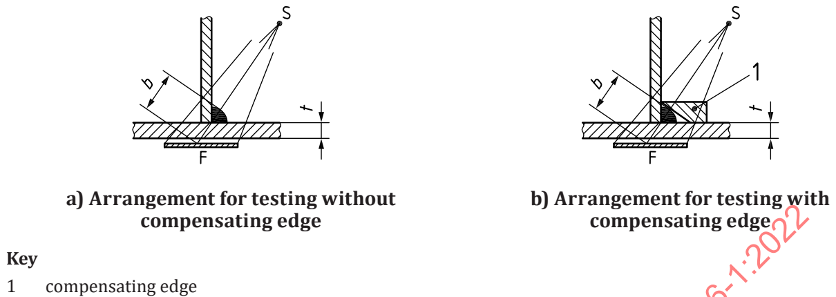
Figure 17 — Arrangement for testing of fillet welds with an oblique film position
