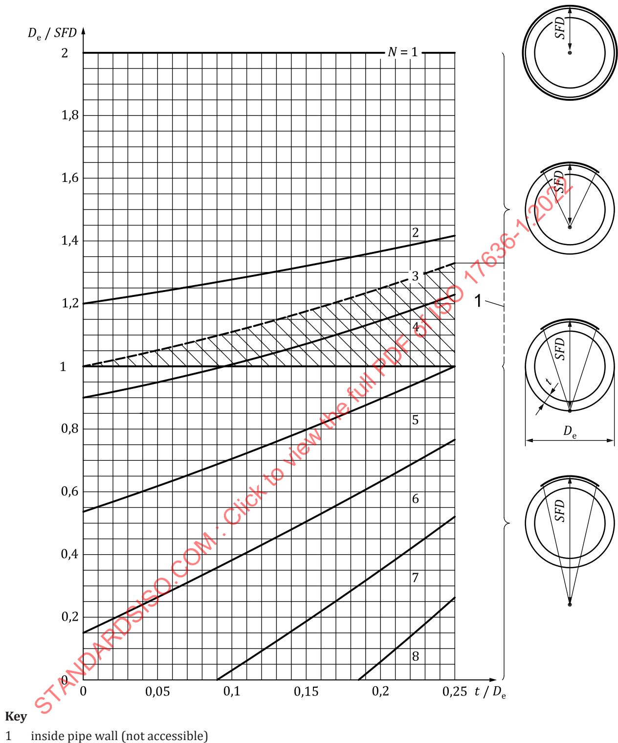
Figure A.4 — Minimum number of exposures N for off-centre penetration with source inside and for double-wall penetration considering a maximum permissible increase in penetrated thickness \Delta t/t = 20\% (testing class A) as a function of ratios t/D_e and D_e/SFD , due to inclined penetration in the evaluable areas of sufficient optical density
