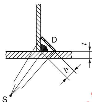
Figure 18 —Test arrangement for penetration of fillet welds
