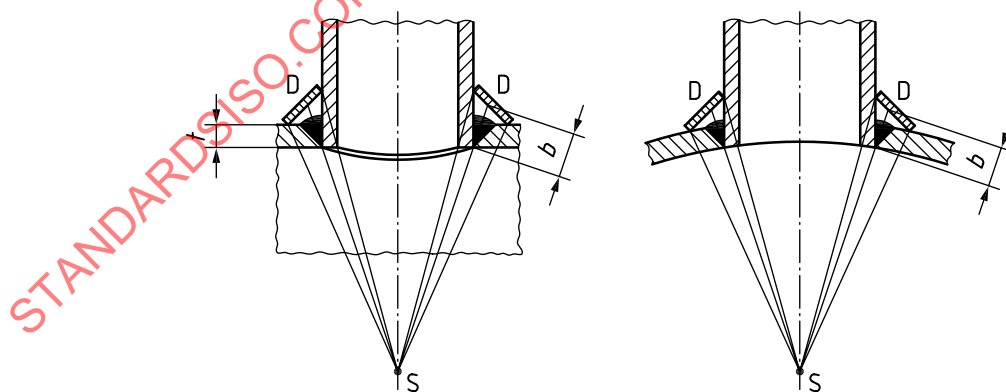
Figure 6 — Arrangement for testing of set-in welds with a radiation source, located on the central pipe axis and perpendicular to the weld centre, and the detector outside
