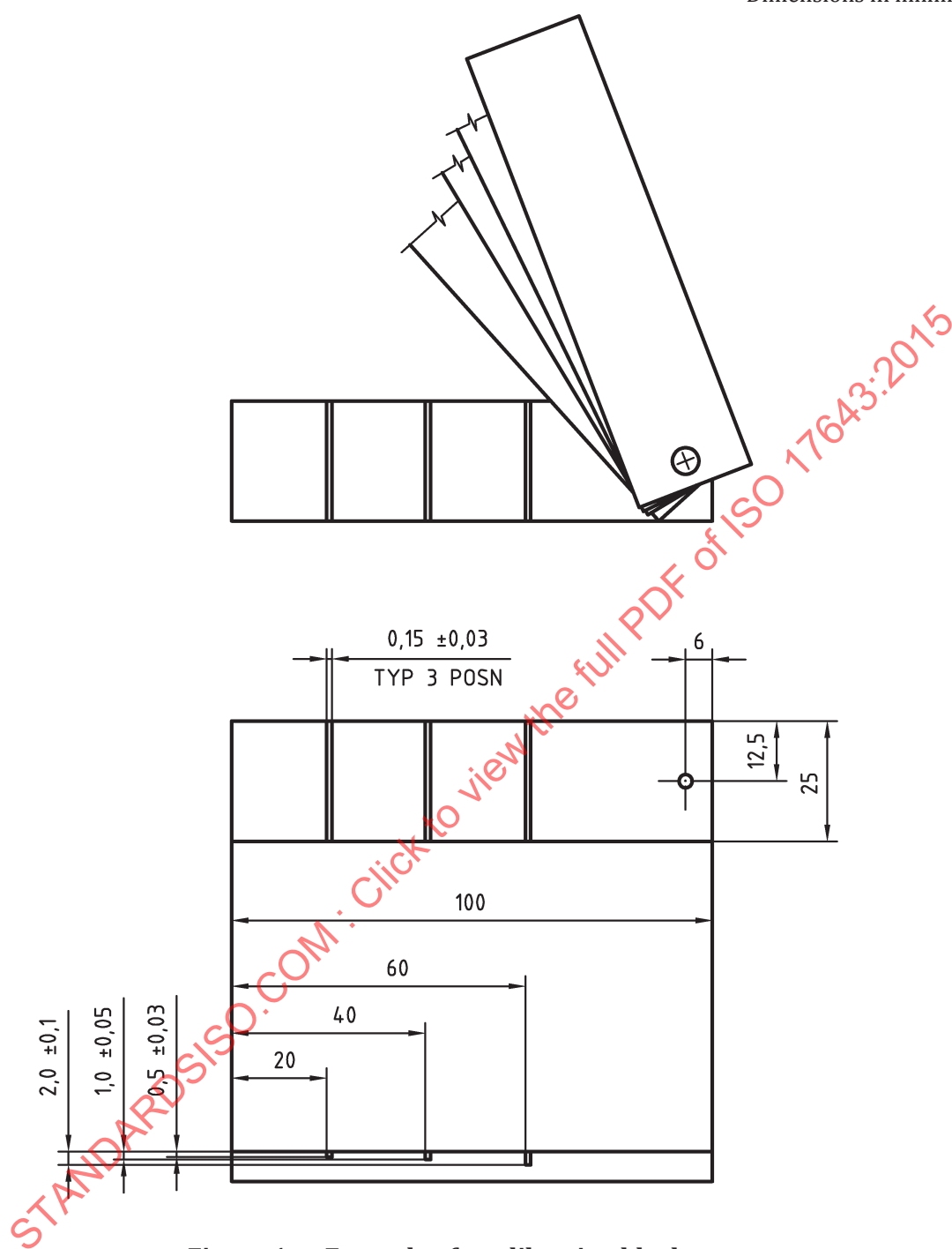
Figure 1 — Example of a calibration block
