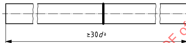
Figure C.1 — Test specimen for butt joint (tensile and bend test)
