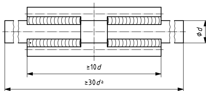
Figure C.3 — Test specimen for strap joint (tensile test)
