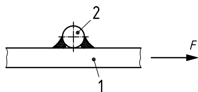
a) Double-sided weld
