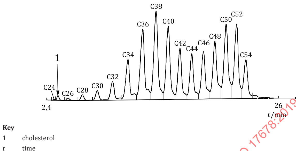
Figure 1 — Example of a triglyceride chromatogram of milk fat with baseline set correctly
