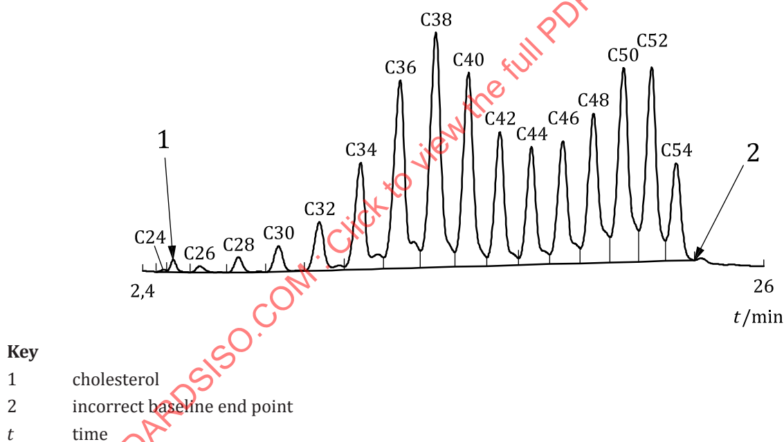
Figure 2 — Example of a triglyceride chromatogram of milk fat with baseline set incorrectly
