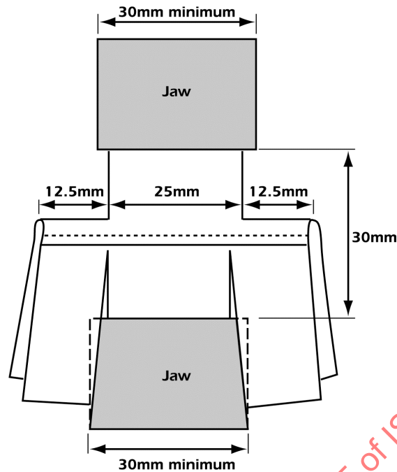
Figure 4 — Clamped test specimen
