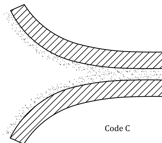
Figure 7 — Defective cohesion
