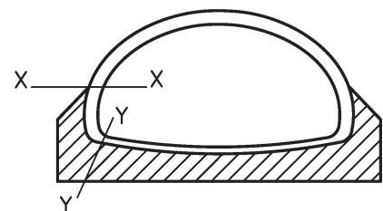
Type d: Strobel stitched
