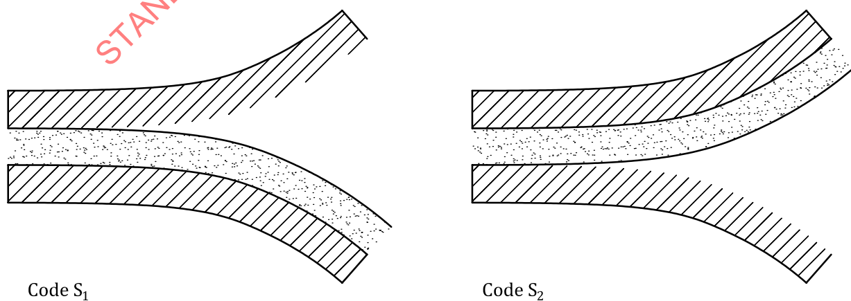
Figure 9 — Material delamination
