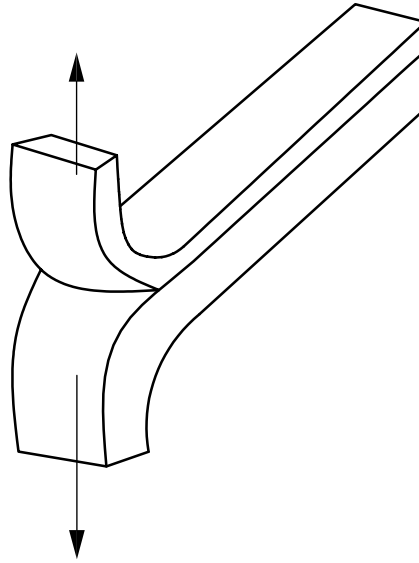
Figure 3 — Prepared test piece
