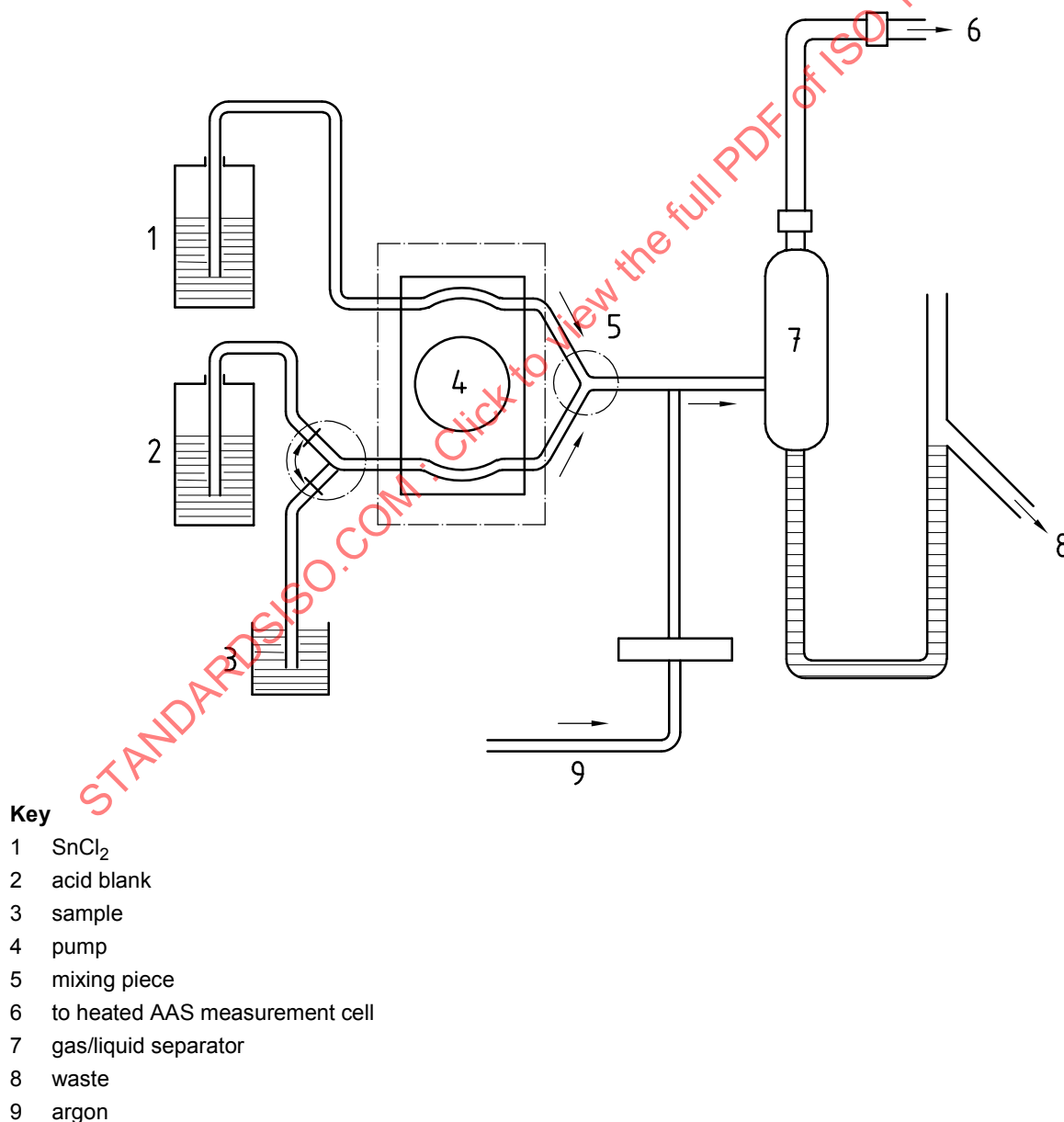
Figure 4 — Schematic diagram of a typical continuous flow CVAAS system
