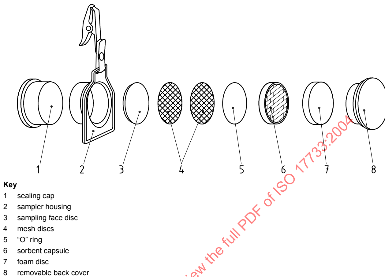
Figure 1 — Mercury diffusive badge
