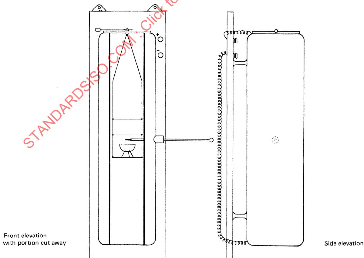
FIGURE — Suitable apparatus for test for resistance to heat and sudden change of temperature
