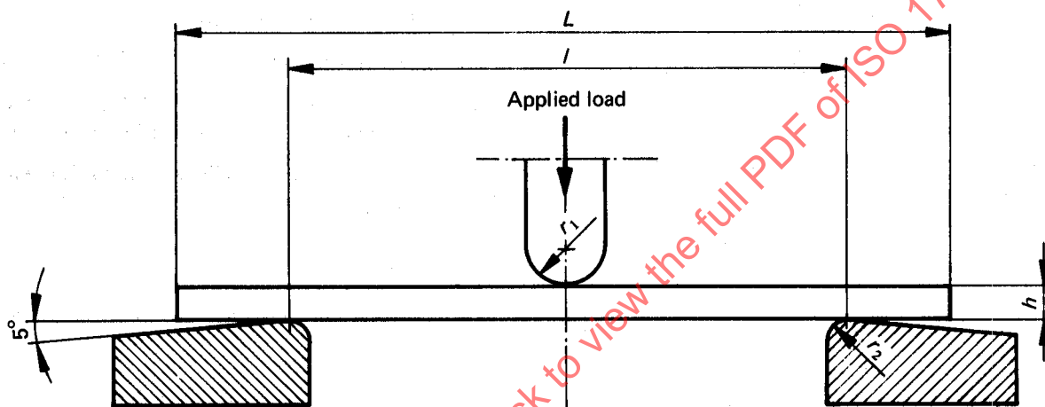
FIGURE 2 — Position of test piece during test
