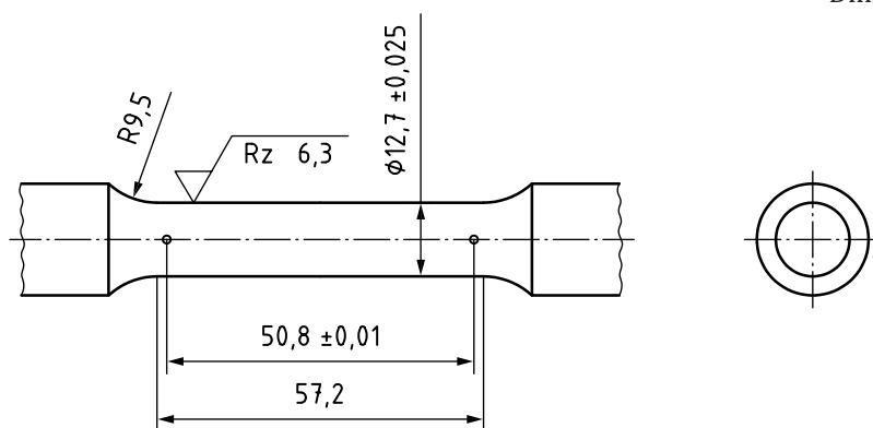
Figure B.1 — Tensile test piece with a gauge length L_0 = 4 \times d
