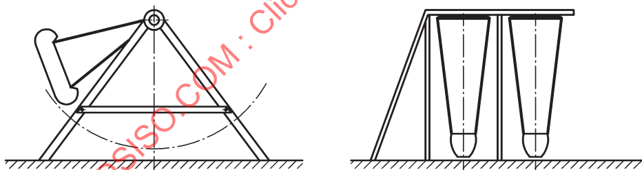
Figure 28 — Main horizontal axis (passenger unit not pivoting and without mechanical drive)
