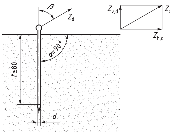
Figure 2 — Rod anchor
