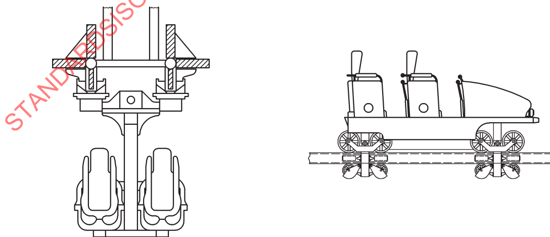
Figure 29 — Track-guided devices
