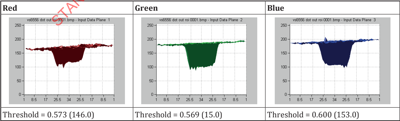
Figure B.3 — Unprocessed ROI dot data
