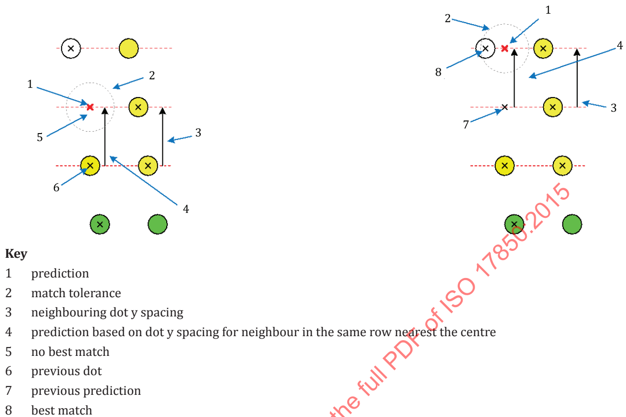
Figure D.7 — Pass 2: handling missing grid points
