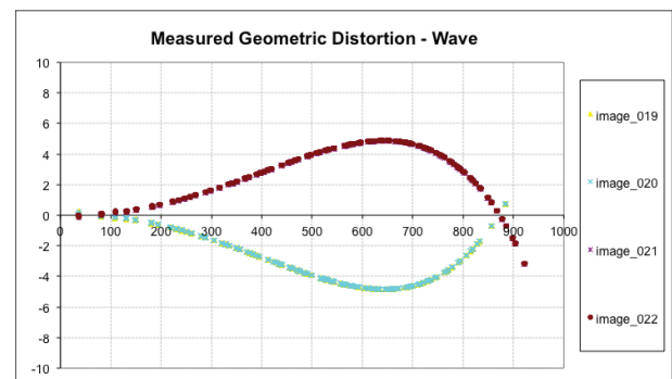
Figure A.1 — Reference images: simulated vs. measured geometric distortion values (X-Axis in per mille of image diagonal and Y-Axis in %)
