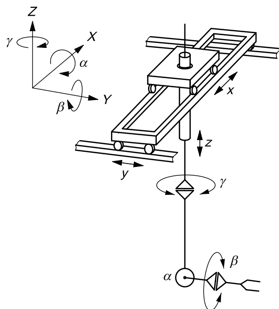
Figure 14 — Remote handling tongs (articulated), horizontal (kinematic diagram)
