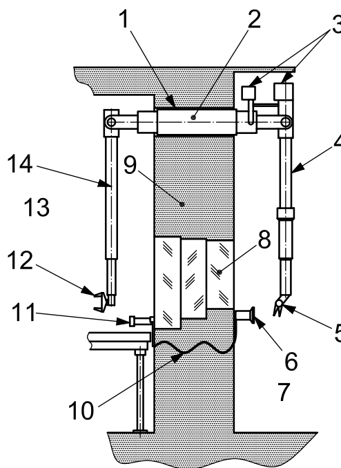
Figure 2 — Mechanical master-slave manipulator with telescopic arms
