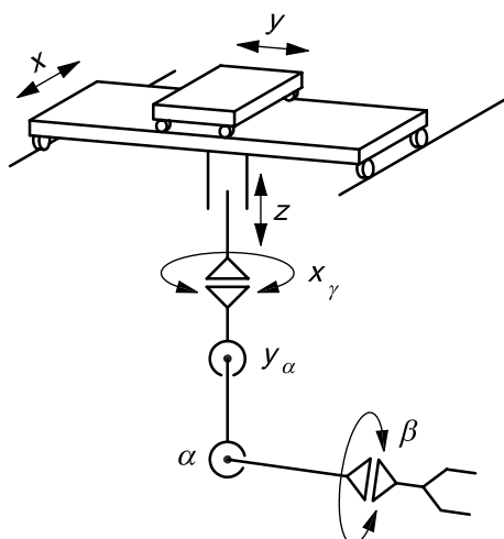
Figure 9 — Power manipulator with preferred design (kinematic diagram)
