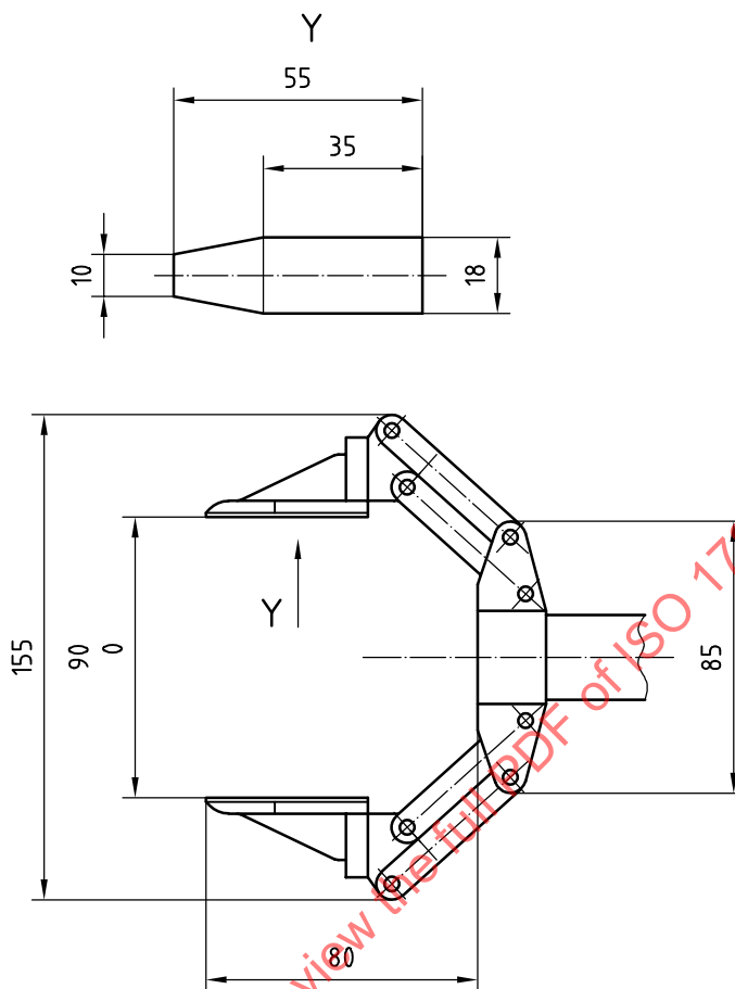
Figure 23 — Dimensions of jaws
