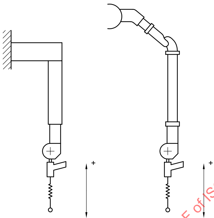
Figure A.3 — Measurement of no-load forces for the Z -motion
