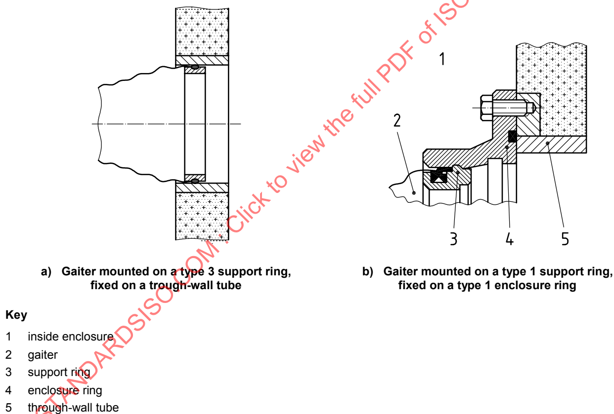
Figure 12 — Gaiter fixed to a through-wall tube
