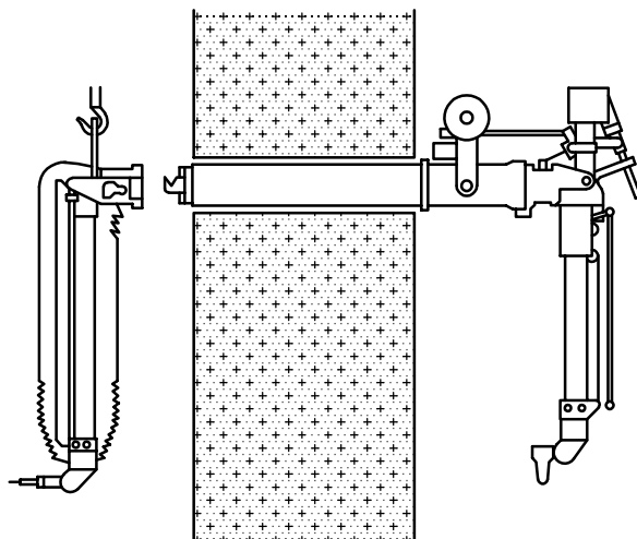
Figure 9 — Fastening of a protection gaiter
