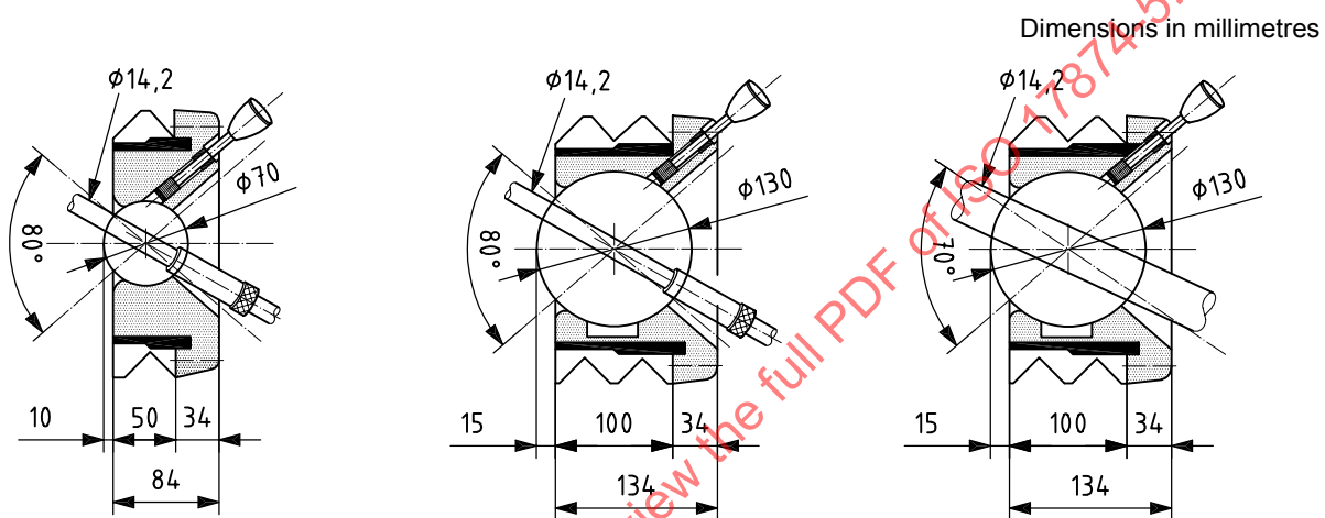
Figure A.1 — Sphere unit Ø 14
