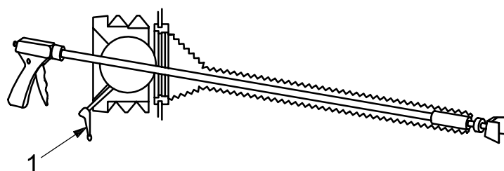
a) Rigid remote handling tongs with gaiter
