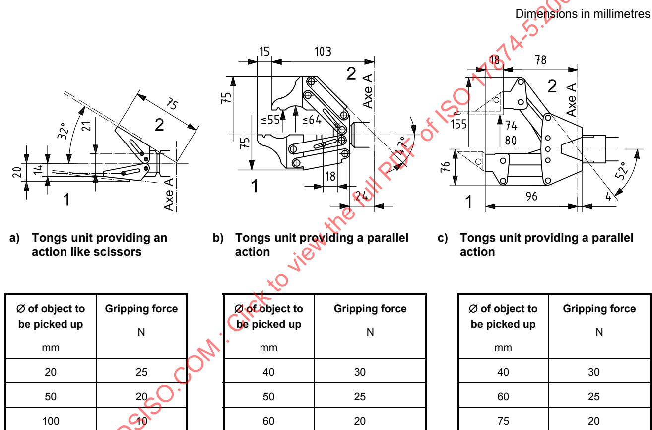
Figure 15 — Tongs units
