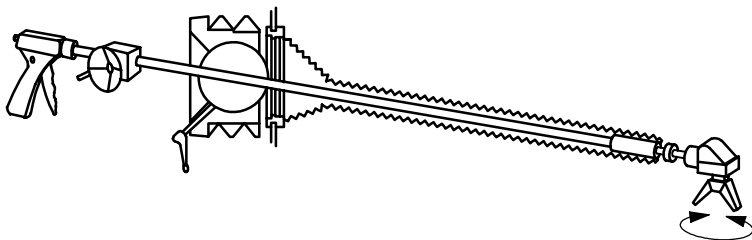
Figure 16 — Remote handling tongs for repetitive movements
