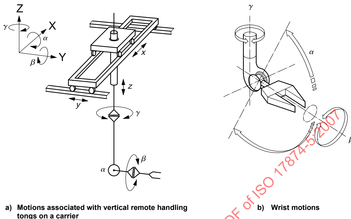
Figure 7 — Vertical remote handling tongs on a carrying system: Kinematics
