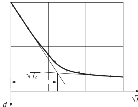
Figure 4 — Example of a time-settlement-curve to determine the time for primary consolidation
