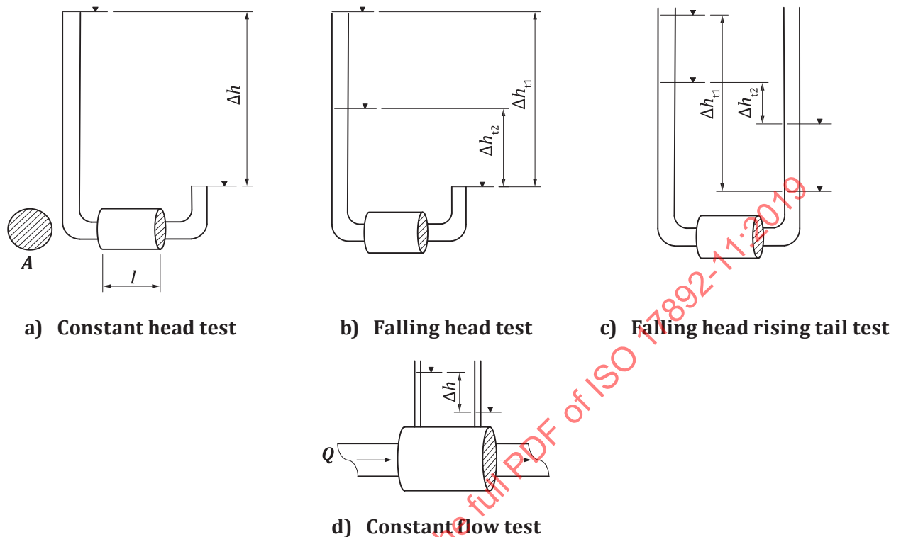
Figure 5 — Alternative arrangements to generate flow for permeability measurement
