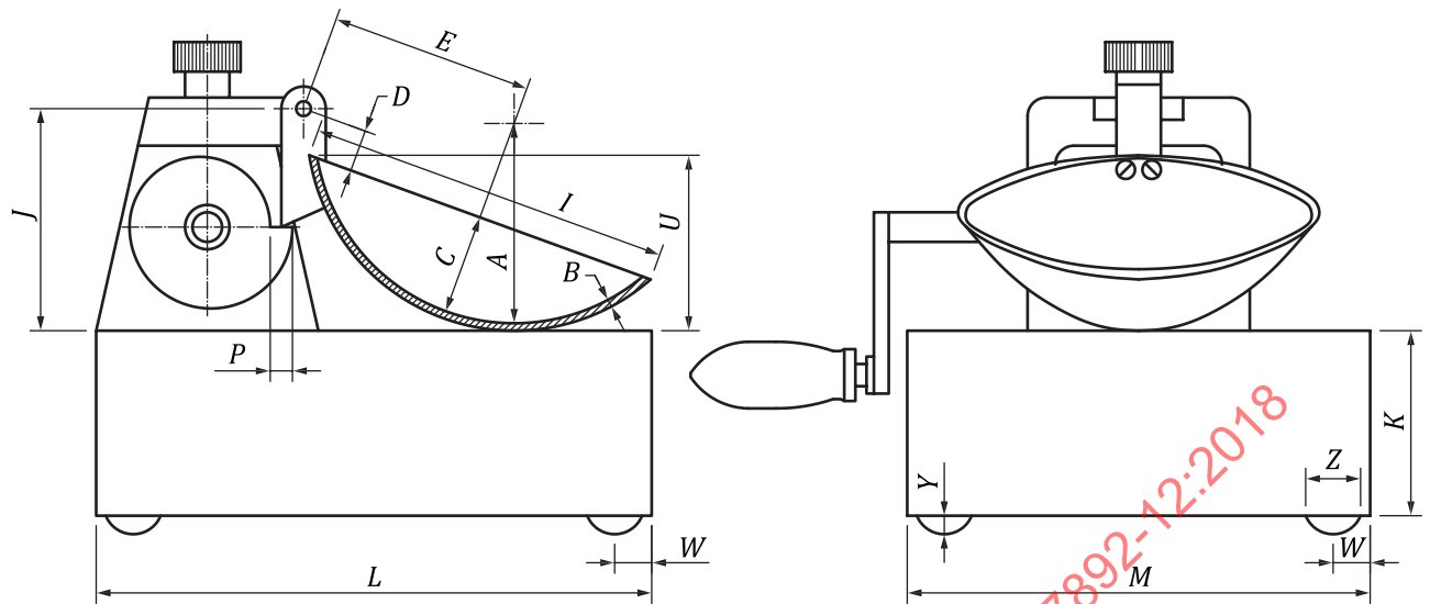
Figure A.2 — Casagrande liquid limit device — Dimensions
