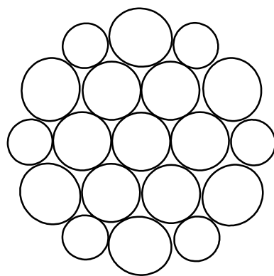
Figure 7 — Warrington construction
