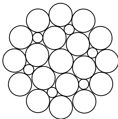
Figure 8 — Filler construction
