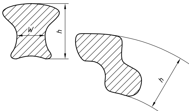
Figure 23 — Half-lock and full-lock wire sections
