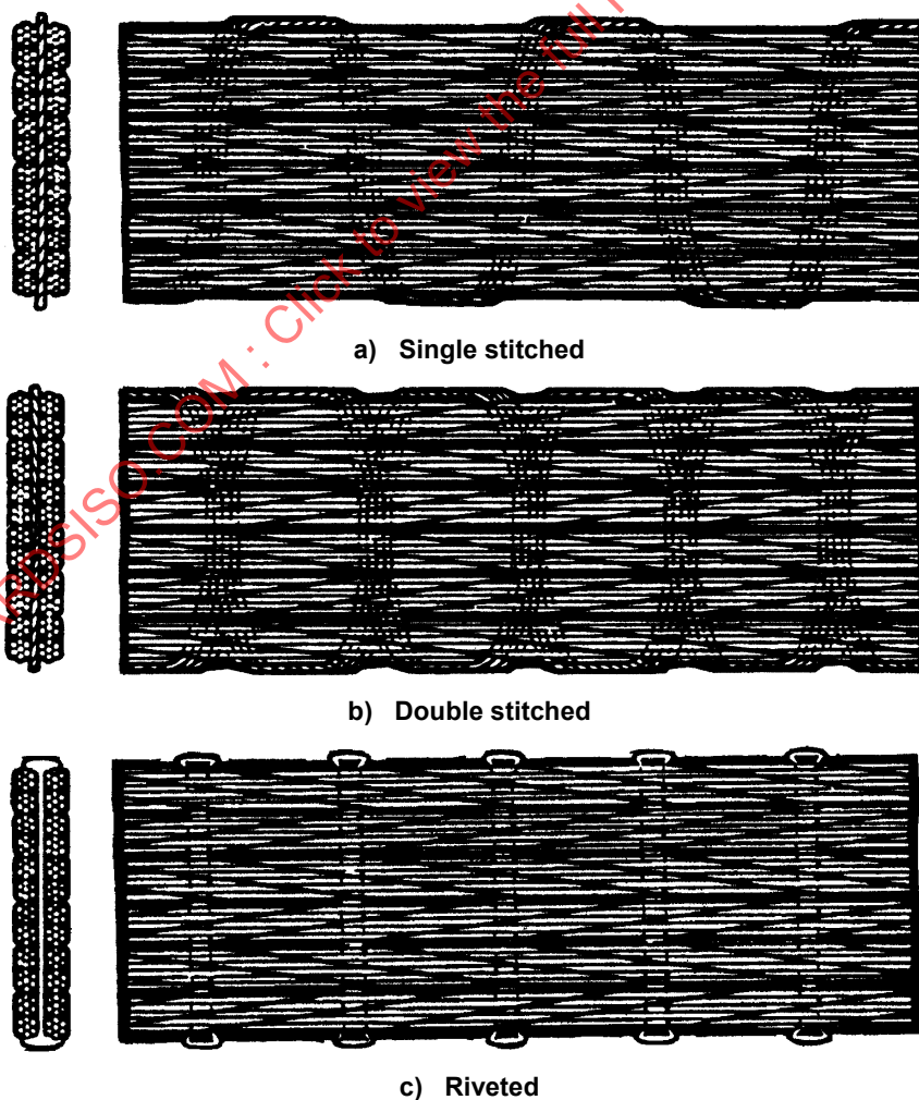
Figure 17 — Examples of flat rope with different stitching
