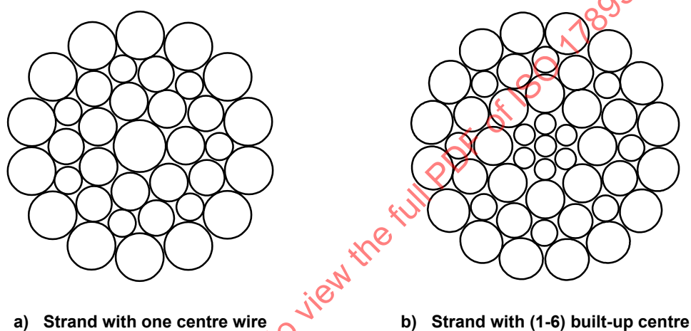
Figure 1 — Round strand with different centres
