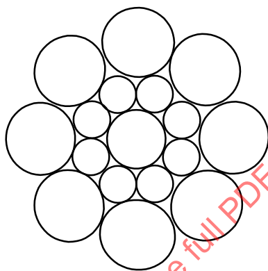
Figure 6 — Seale construction
