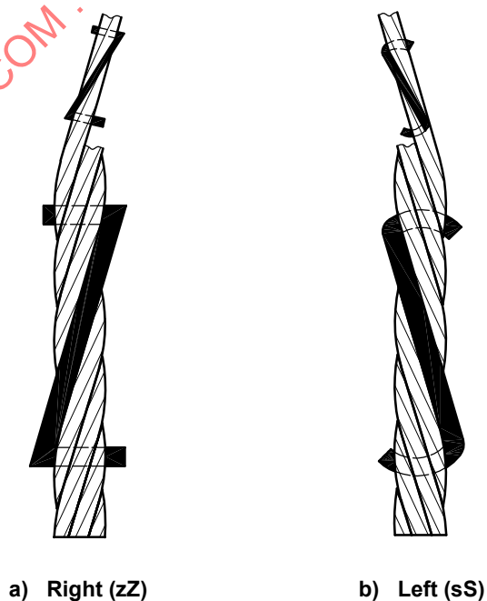
Figure 32 — Lang lay
