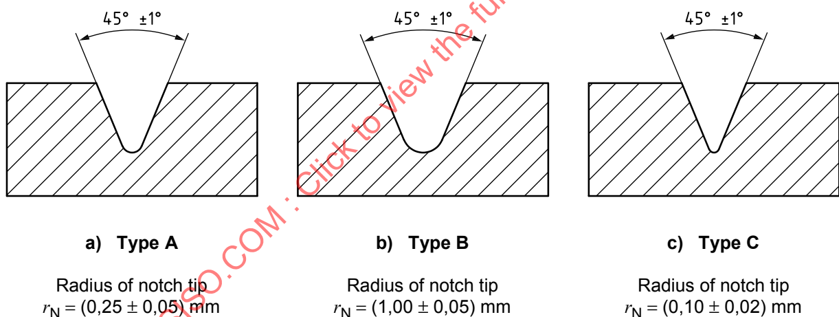
Figure 5 — Notch types
