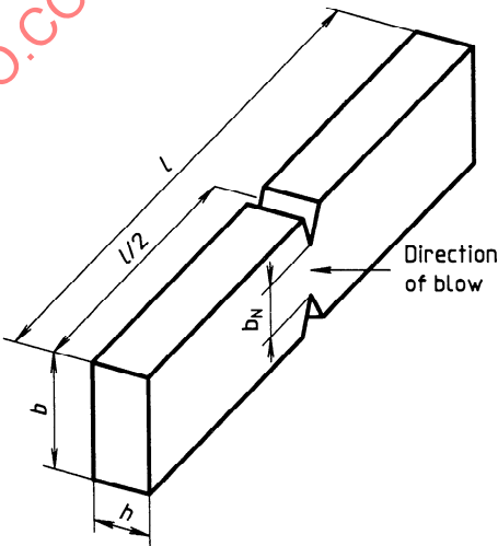
Figure A.1 — Charpy flatwise impact (f) with double-notched specimen
