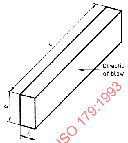
Figure 3 — Charpy flatwise impact (f)
