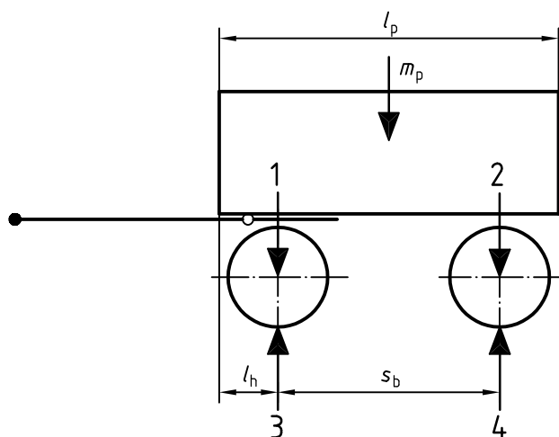
Figure 3 — Balanced trailer
