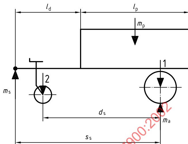
Figure 1 — Semi-mounted trailer
