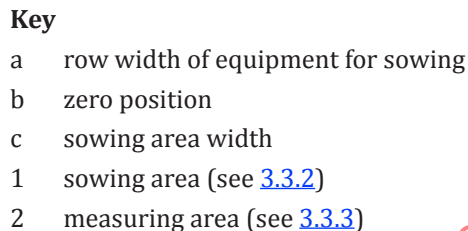
Figure 2 — Sowing area and measuring area set-up
