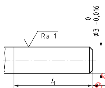
Figure 7 — Dimensions Type 4 shank
