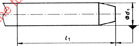
Figure 3 — Type 3 shank
