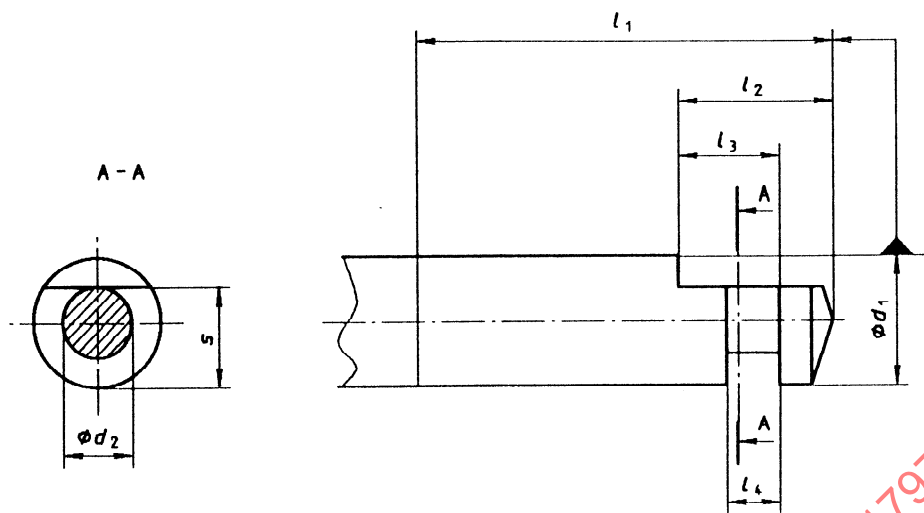
Figure 1 — Type 1 shank
