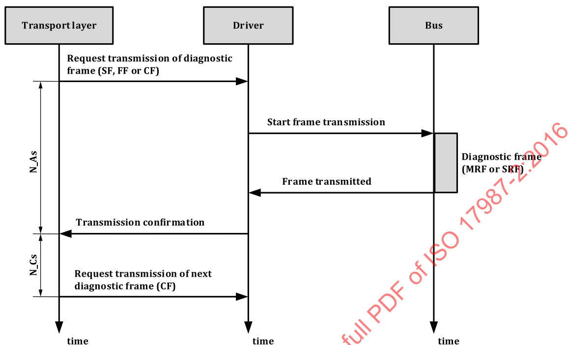
Figure 11 — Transport layer timing on transmitter side
