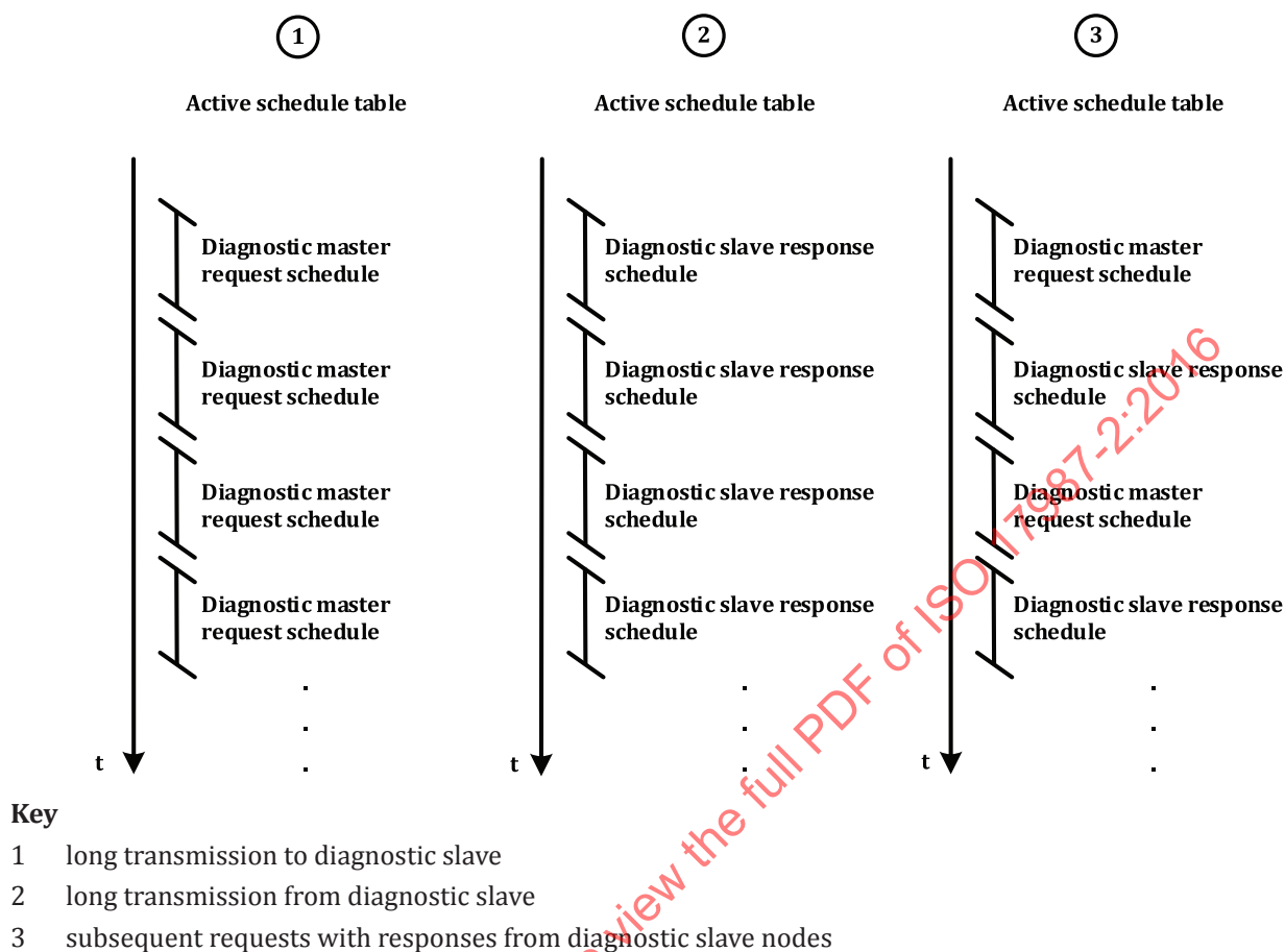
Figure 25 — Use cases for diagnostic only mode
