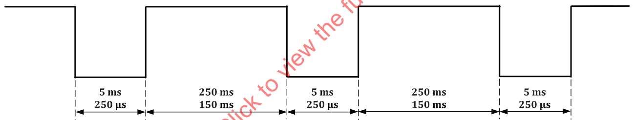
Figure 4 — One block of wake up signals
