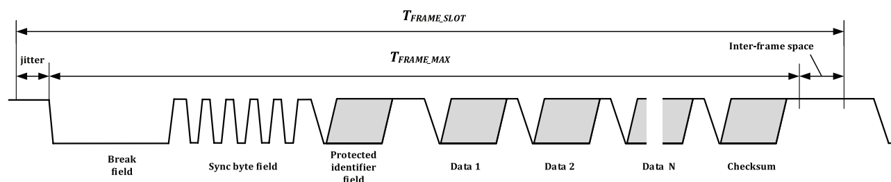
Figure 17 — Frame slot
