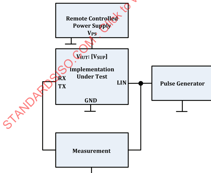
Figure 5 — Test system: IUT as receiver V_{SUP} at V_{BUS\_rec} (up)
