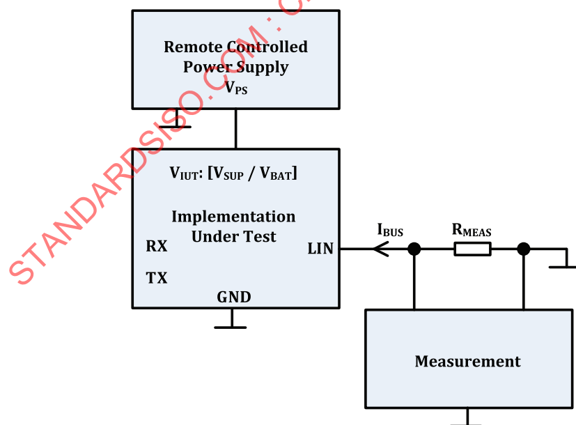
Figure 51 — Test system: I_{\text{BUS\_PAS\_dom}} IUT in recessive state V_{\text{BUS}} = 0 \text{ V}
