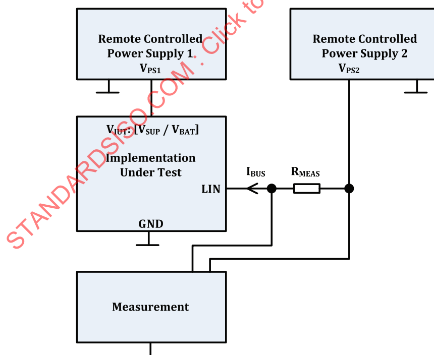
Figure 29 — Test system: I_{\text{BUS\_PAS\_rec}} IUT in recessive state: V_{\text{BAT}} = 8,0 \text{ V} with variation of V_{\text{BUS}} \in [8,0 \text{ V to } 18 \text{ V}]
