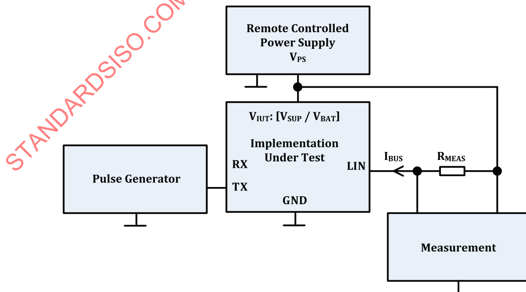
Figure 50 — Test system: I_{BUS\_LIM} at dominant state (driver on)
