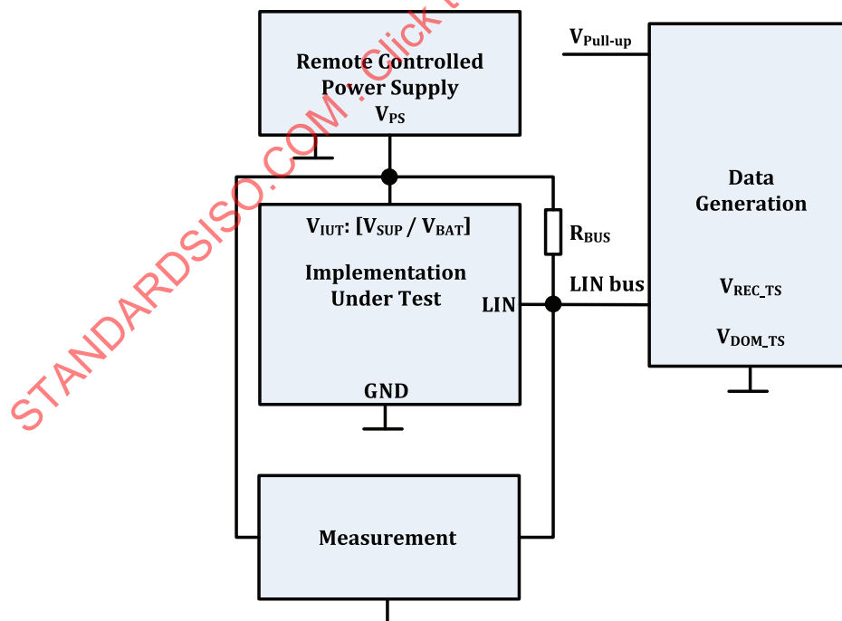
Figure 69 — Test system: I_{BUS\_LIM} at dominant state (driver on)
