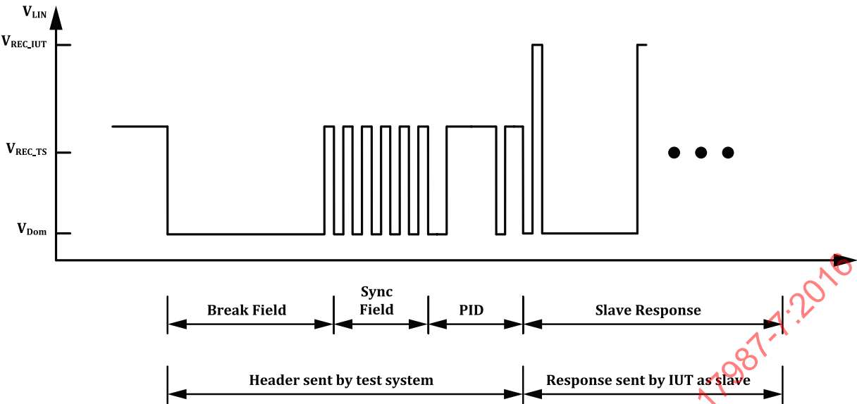
Figure 21 — LIN header sent by test system as master with recessive voltage ( V_{\text{Rec\_TS}} ) adjusted and IUT as slave answering with nominal recessive voltage ( V_{\text{Rec\_IUT}} )
