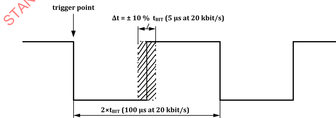
Figure 44 — RX response of test system: Operating voltage range
