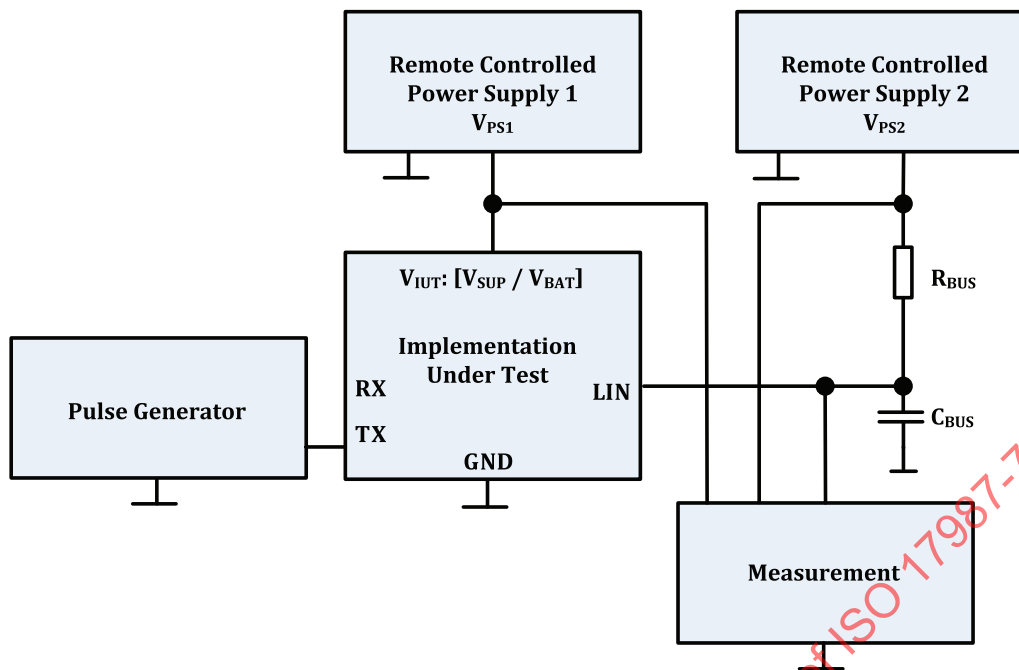
Figure 54 — Test system: Measuring the duty cycle
