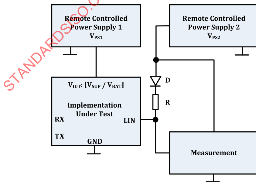
Figure 7 — Test system: Variation of V_{SUP\_NON\_OP}
