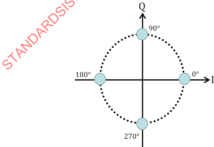
Figure 3 — Transmitter phase's definition
