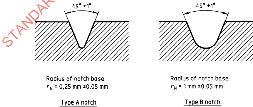
Figure 3 — Notch types
