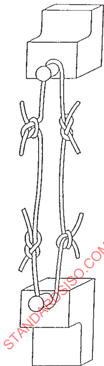
Figure 1 — Mounting of a mesh by pins
