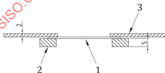
Figure 6. — Side view of turntable
