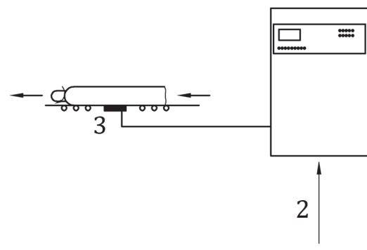
b) UT system with cylinder submerged in water
