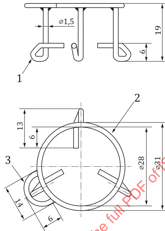
a) Suitable for single determination (top: side view; bottom: top view)
