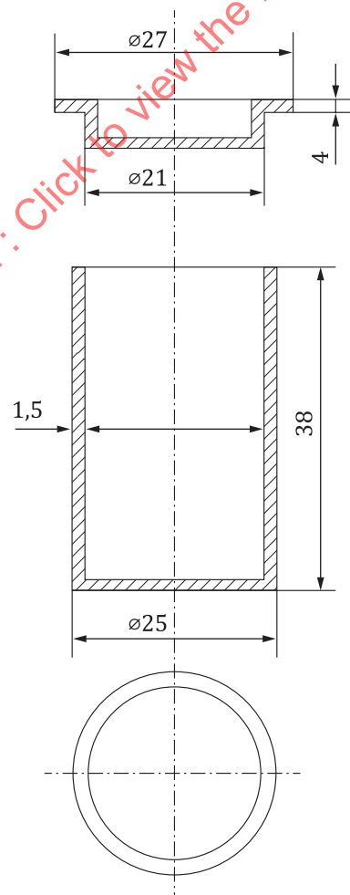
Figure 2 — Silica crucible and lid
