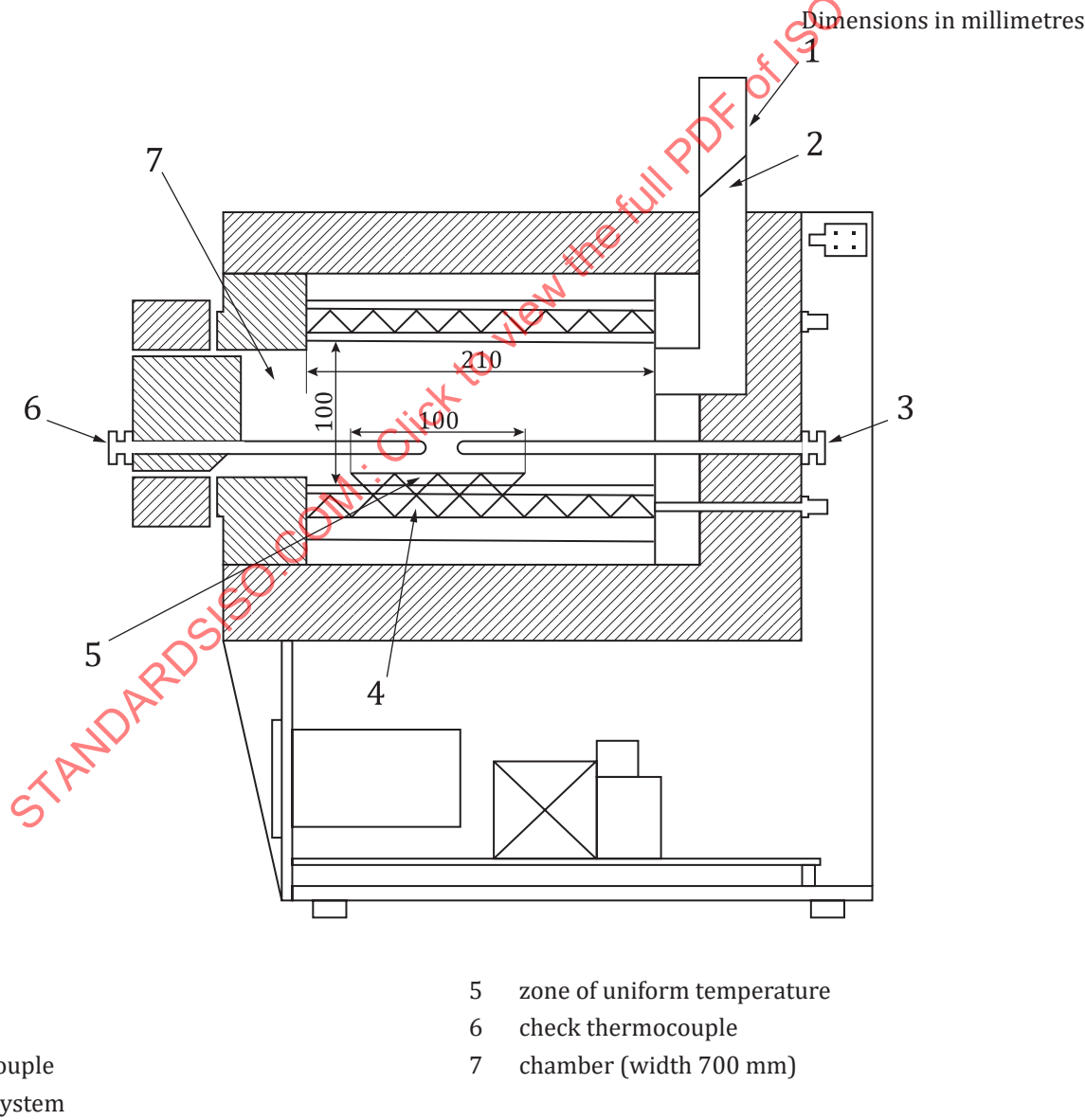
Figure 1 — Example of suitable furnace
