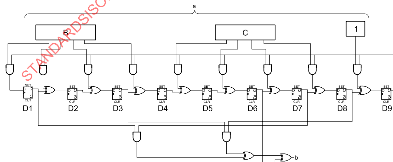
Figure 5 — eSeal transmitter PN generator
