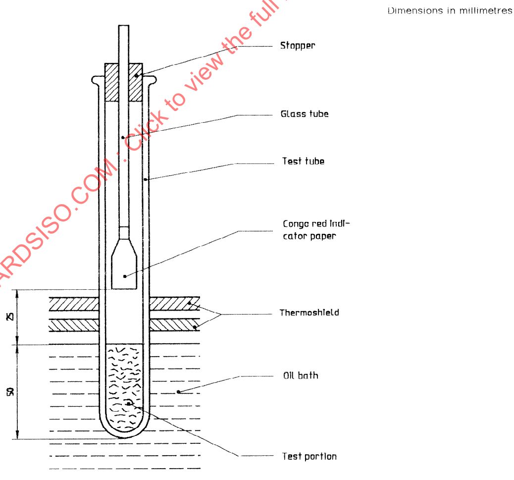
Figure 1 — Arrangement of the test tube in the oil bath
