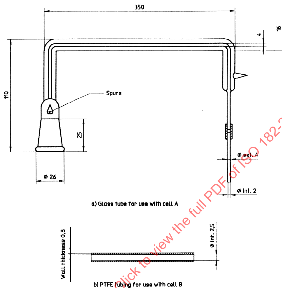
Figure 4 — Tubes for connecting dehydrochlorination cell to measurement cell
