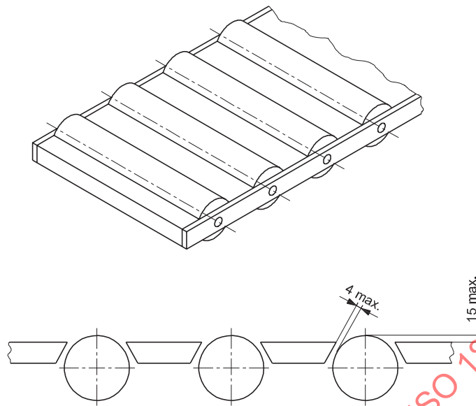
Figure 6 — Safeguarding of gaps between the rollers
