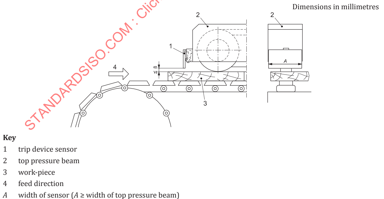
Figure 8 — Trip device at the infeed end of the machine
