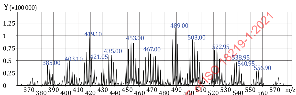
Figure B.1 — Example of chromatogram of SCCPs analysis with LC-MS/MS
