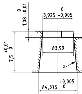
a) Gauge for testing rigid male conical fittings
