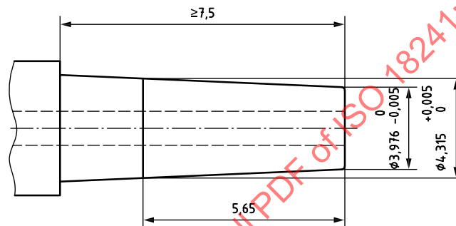
Figure A.5 — Reference steel male conical fitting
