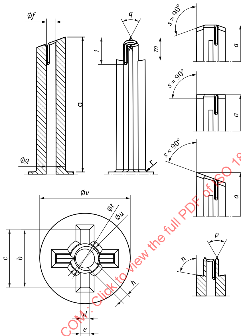
Figure B.2 — Cross connector shaft (E1R)
