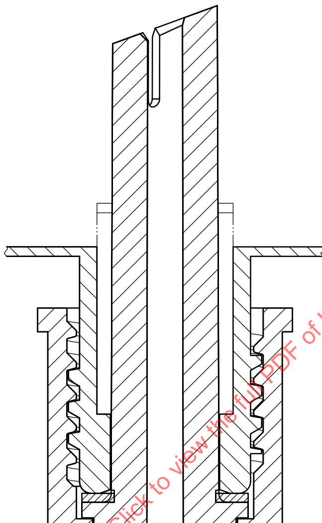
Figure B.4 — Connection of cross connector and cross port reservoir connector (E1R)
